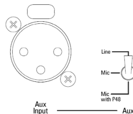
Figure 7 - Rear auxiliary input XLR3
