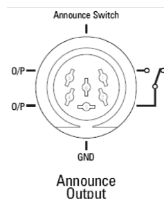
Figure 9 - Rear 6-pin DIN socket
